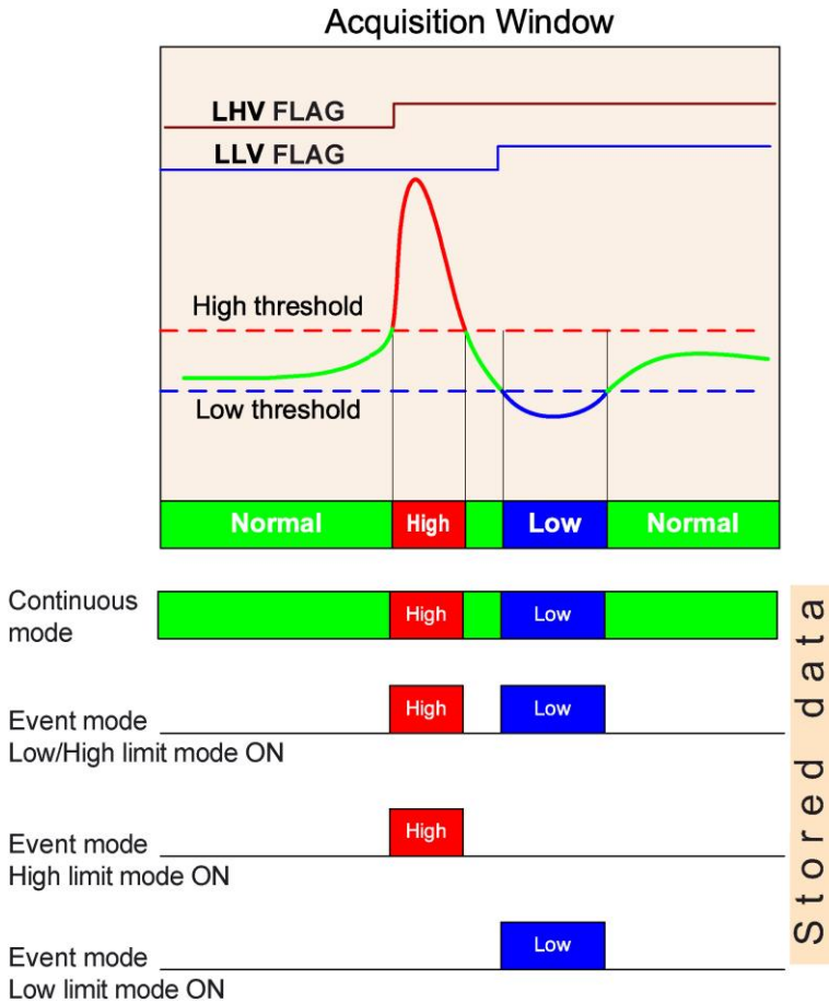
Fig. 2.1: A927ZET Sampling Operating Modes
