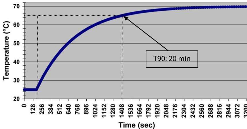
Fig. 4.2: A927ZET Response Time
