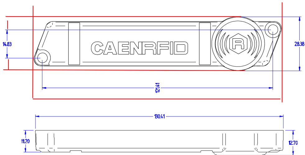
Fig. 1.3: A927ZET Technical drawings
