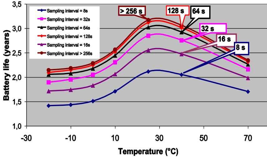
Fig. 4.1: A927ZET Battery life (typ.)
