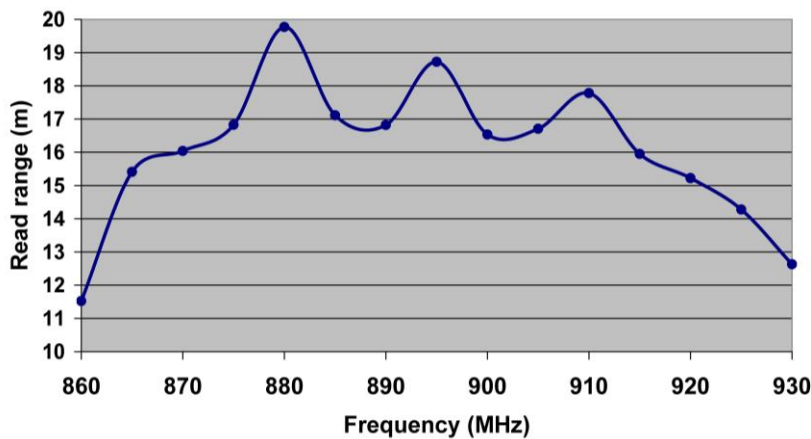
Fig. 4.5: A927ZET Theoretical read range at 2W ERP
