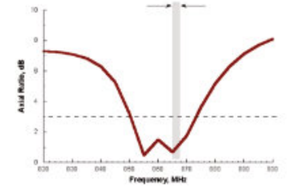
Axial Ratio
